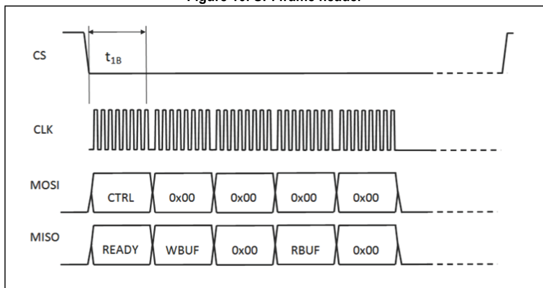
Figure 10. SPI frame header
