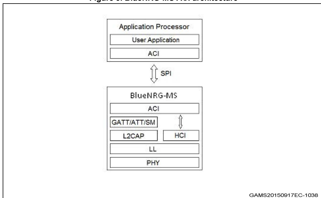
Figure 3. BlueNRG-MS ACI architecture
