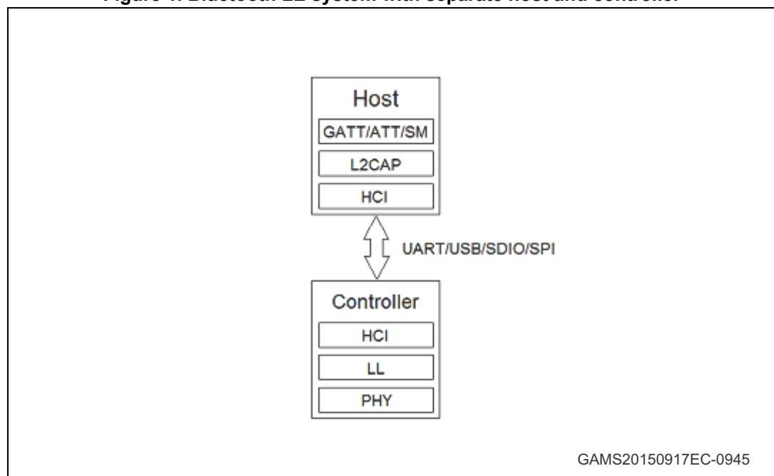
Figure 1. Bluetooth LE system with separate host and controller
